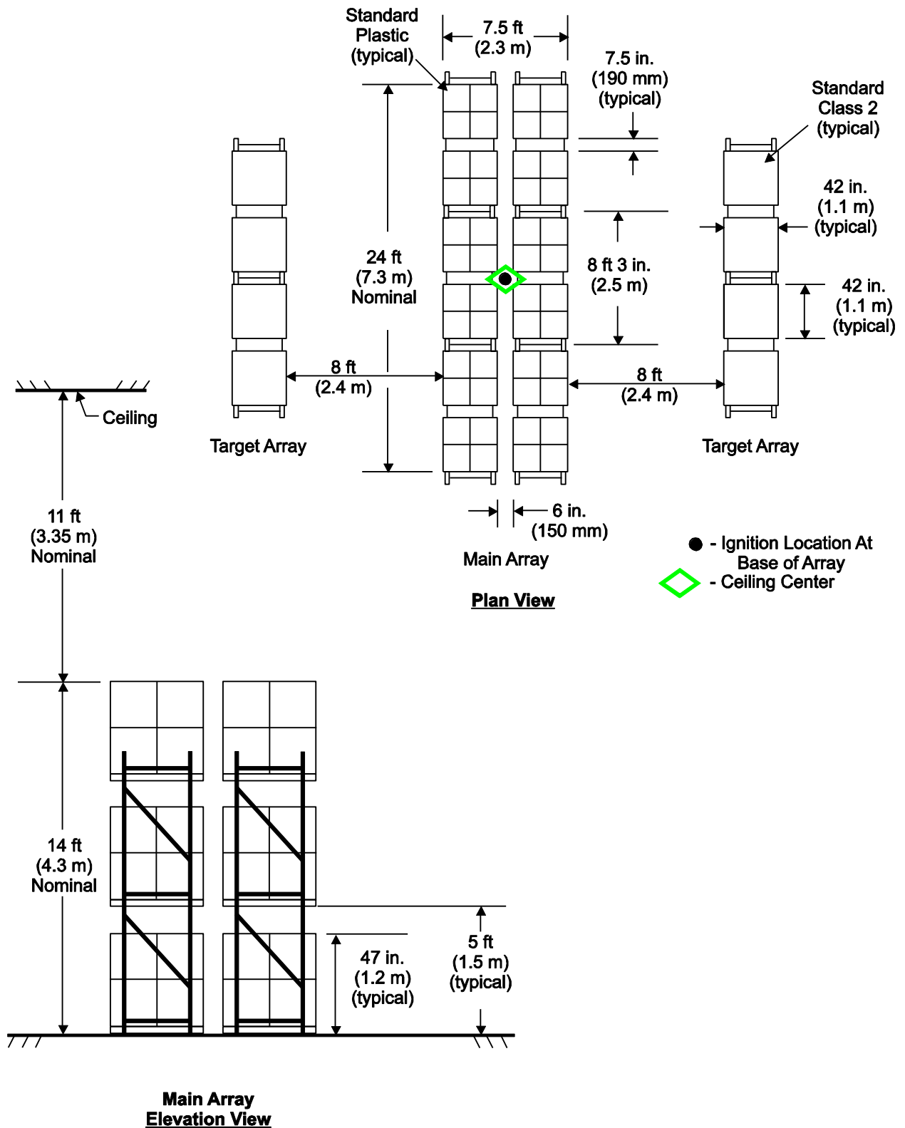
D-34: Full Scale Fire Test Array for K16.8 (K240) Upright Storage Sprinkler, Test B
