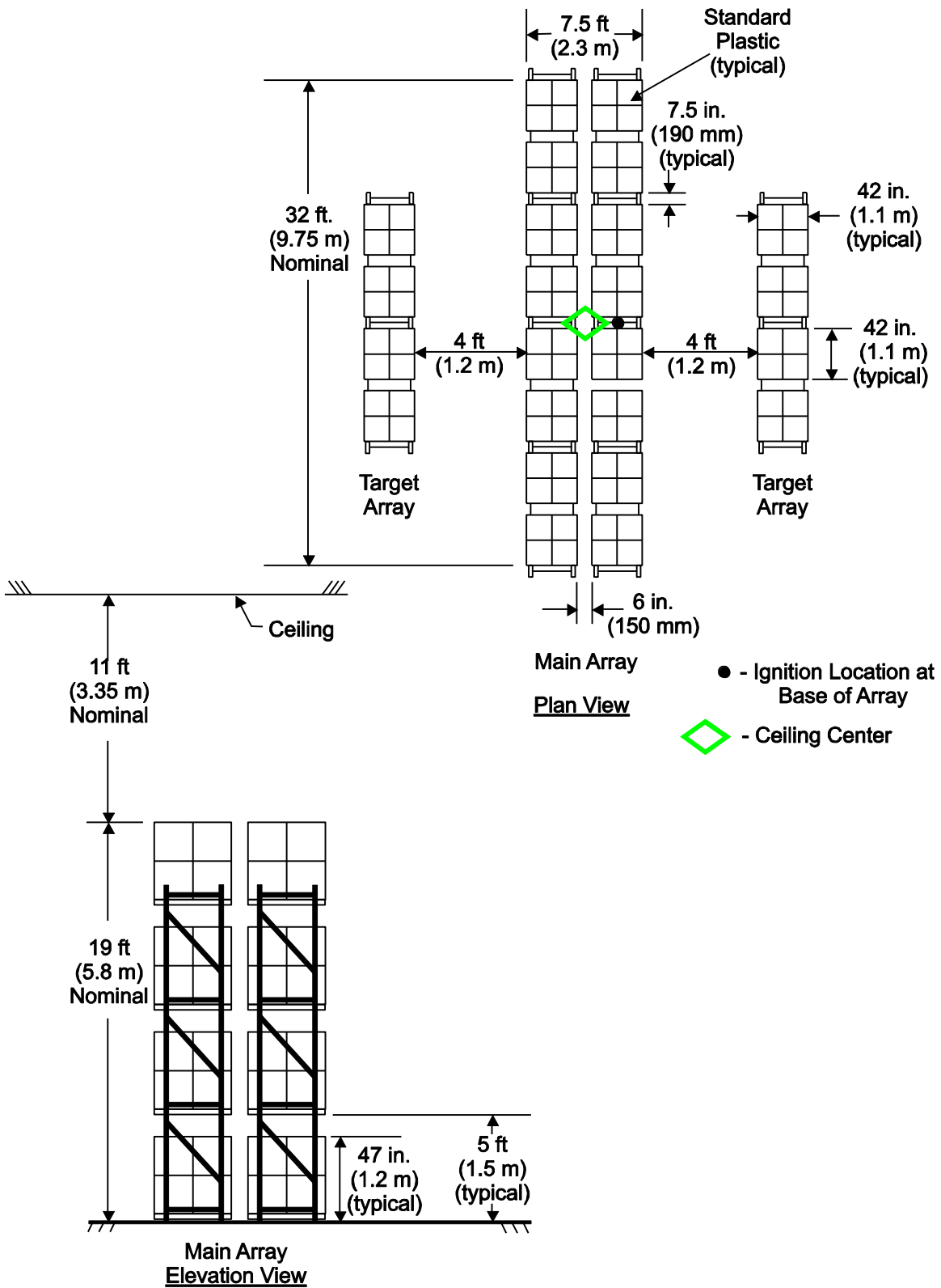
D-35: Full Scale Fire Test Array for K19.6 (K280) Pendent Sprinkler, Test A and B
