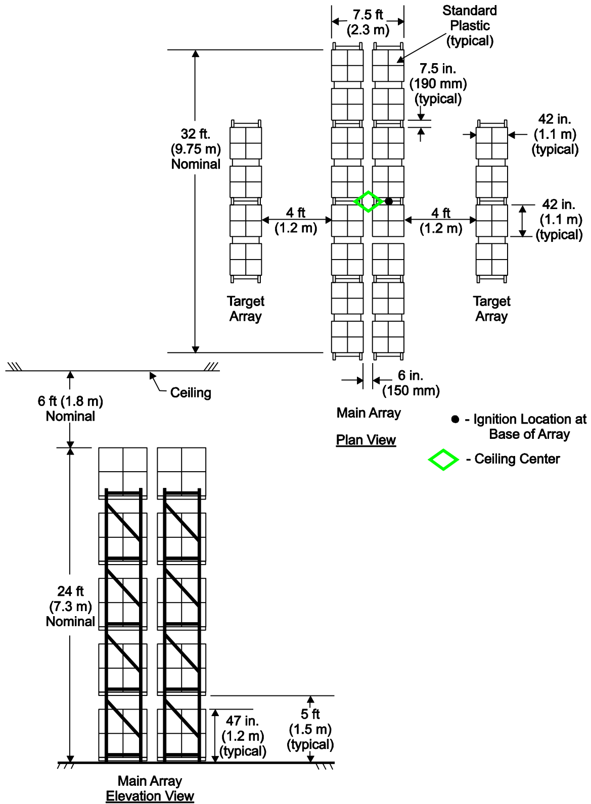
D-36: Full Scale Fire Test Array for K19.6 (K280) Pendent Sprinkler, Test C
