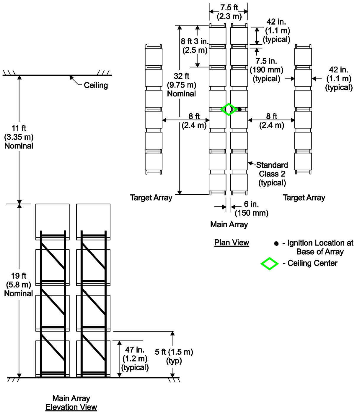
D-24: Full Scale Fire Test Array for K11.2 (K160) and K14.0 (K200) Upright and Pendent Storage Sprinklers, Test A
