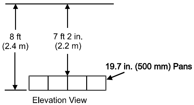
D-17: Distribution Test Setup for Extended Coverage Hazard Category 1 (HC-1) Sprinklers
