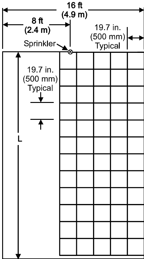
Plan View EC Sidewall
