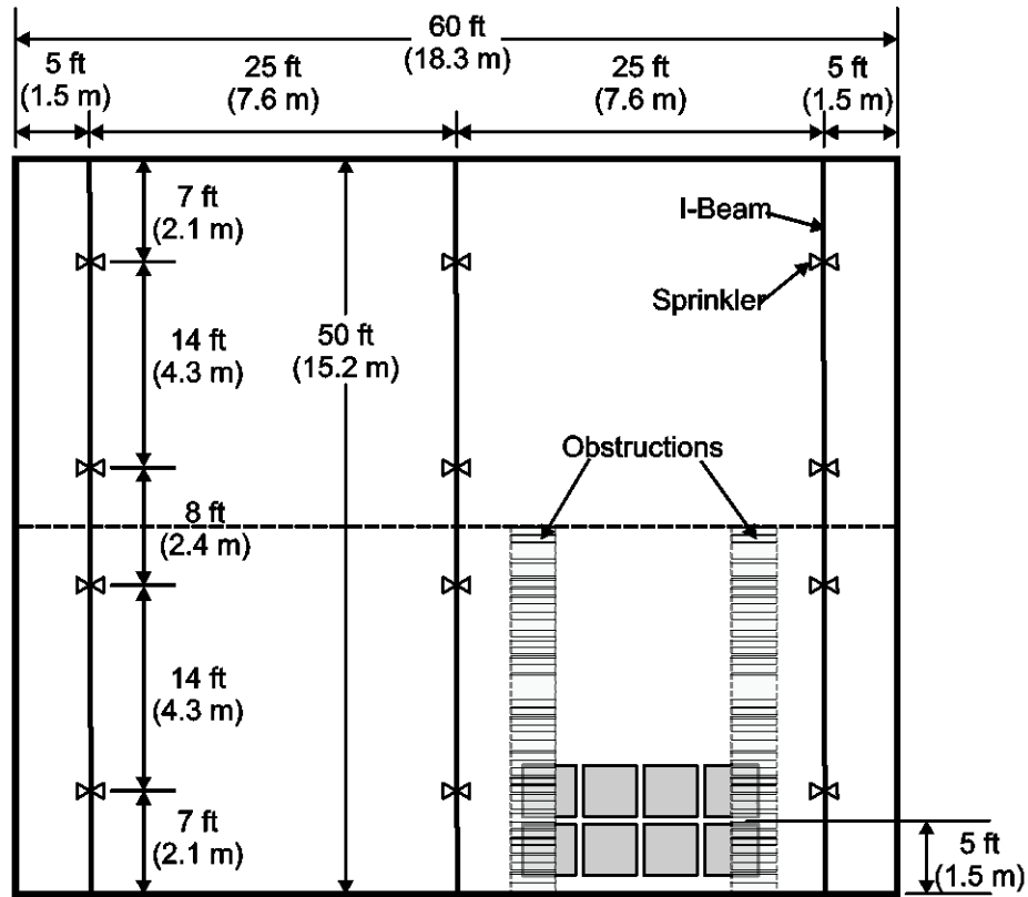
Plan View Obstruction Tests A and B
