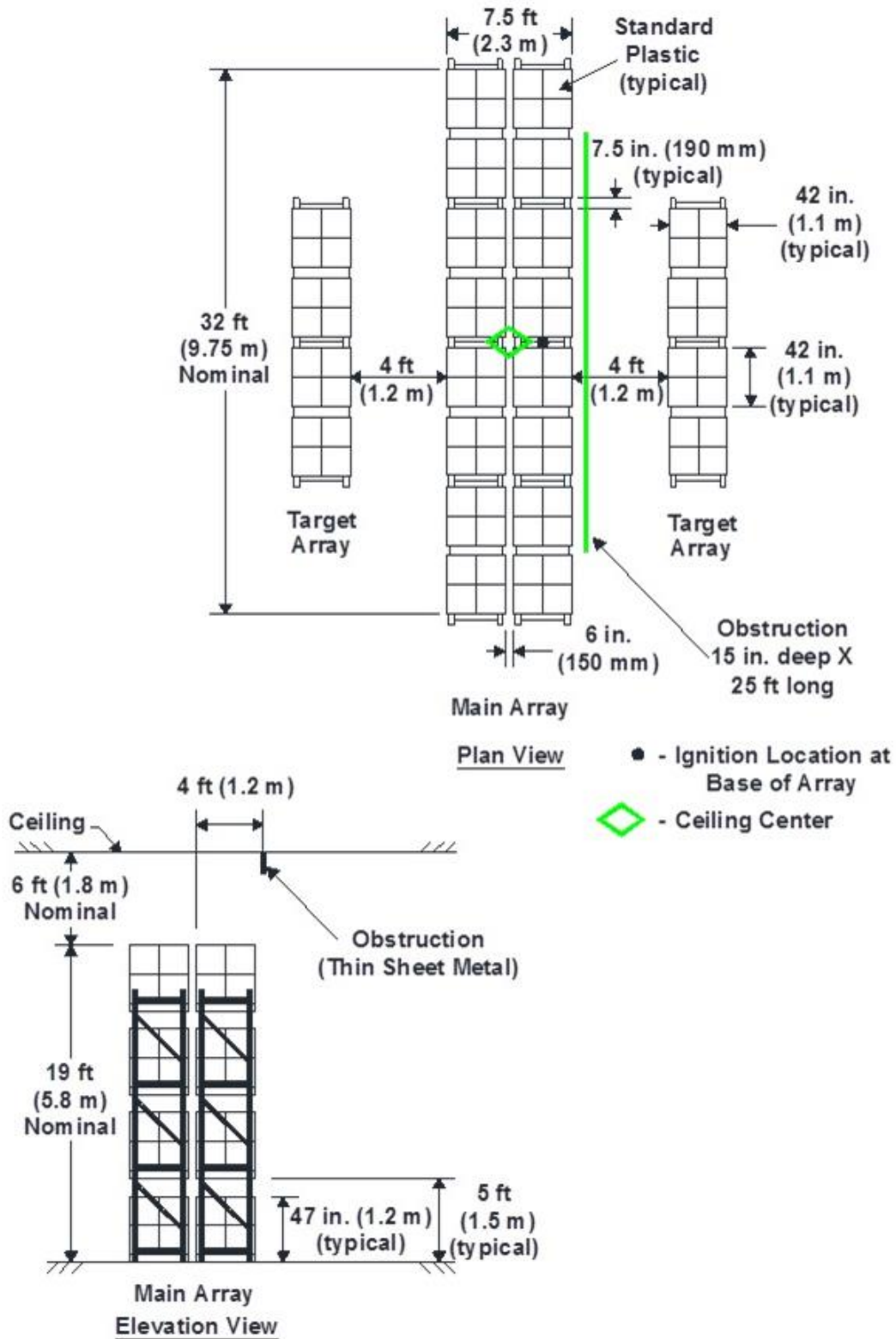
D-43: Full Scale Fire Test Array for K25.2 EC (K360EC) Upright and Pendent Sprinklers, Test D
