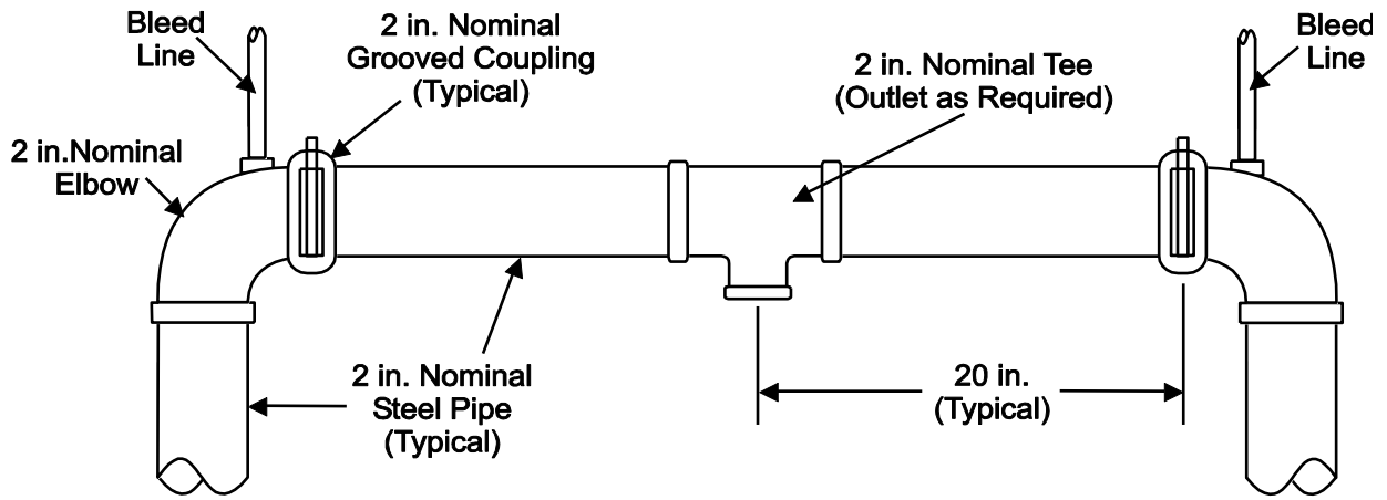
Test Apparatus for Double-Fed Flow
