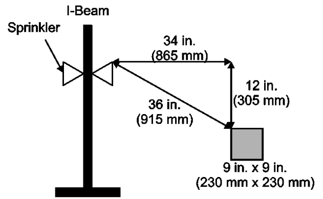
End Elevation View 9 in. (230 mm) Wide Obstruction 36 in. (915 mm) Separation
