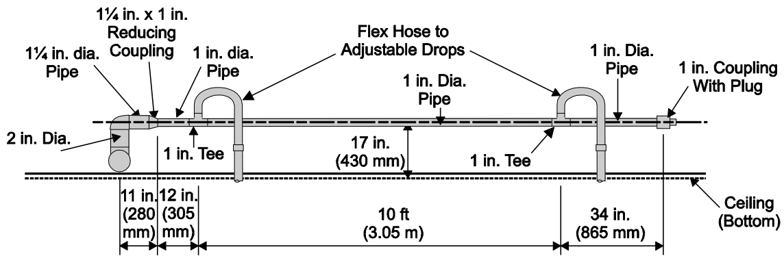
Typical Branch Line
