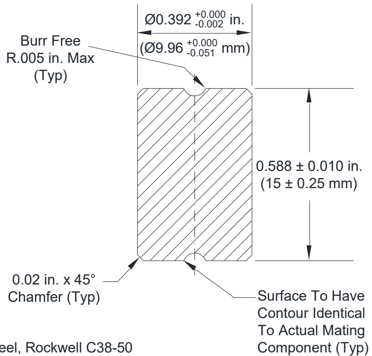
D-3: Bulb Crush Inserts for Strength of Element Test
