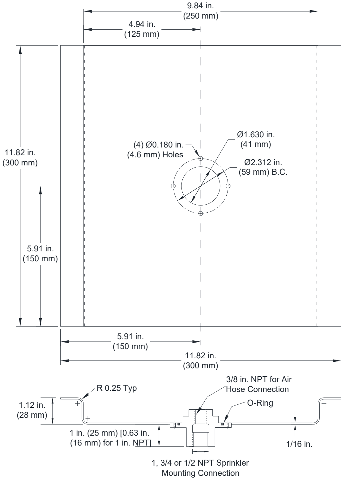
D-9: Plunge Tunnel Test Plate (For Sensitivity - RTI Test)
