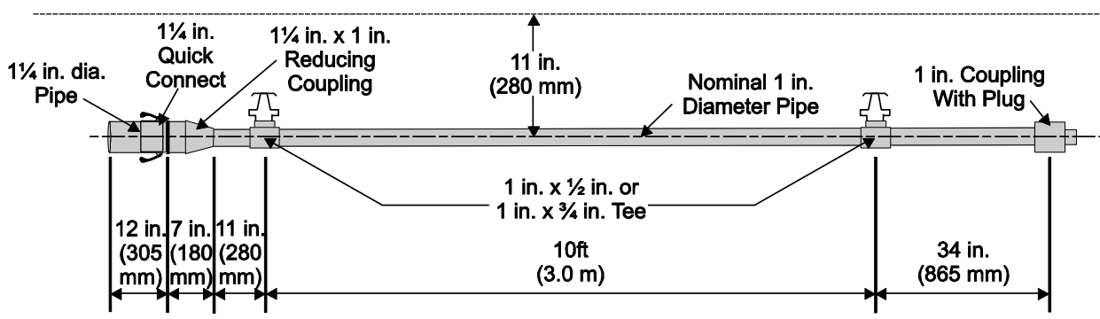
Typical Branch Line
