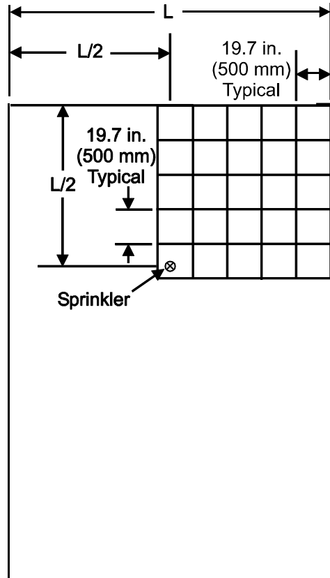
Plan View EC Upright and Pendant
