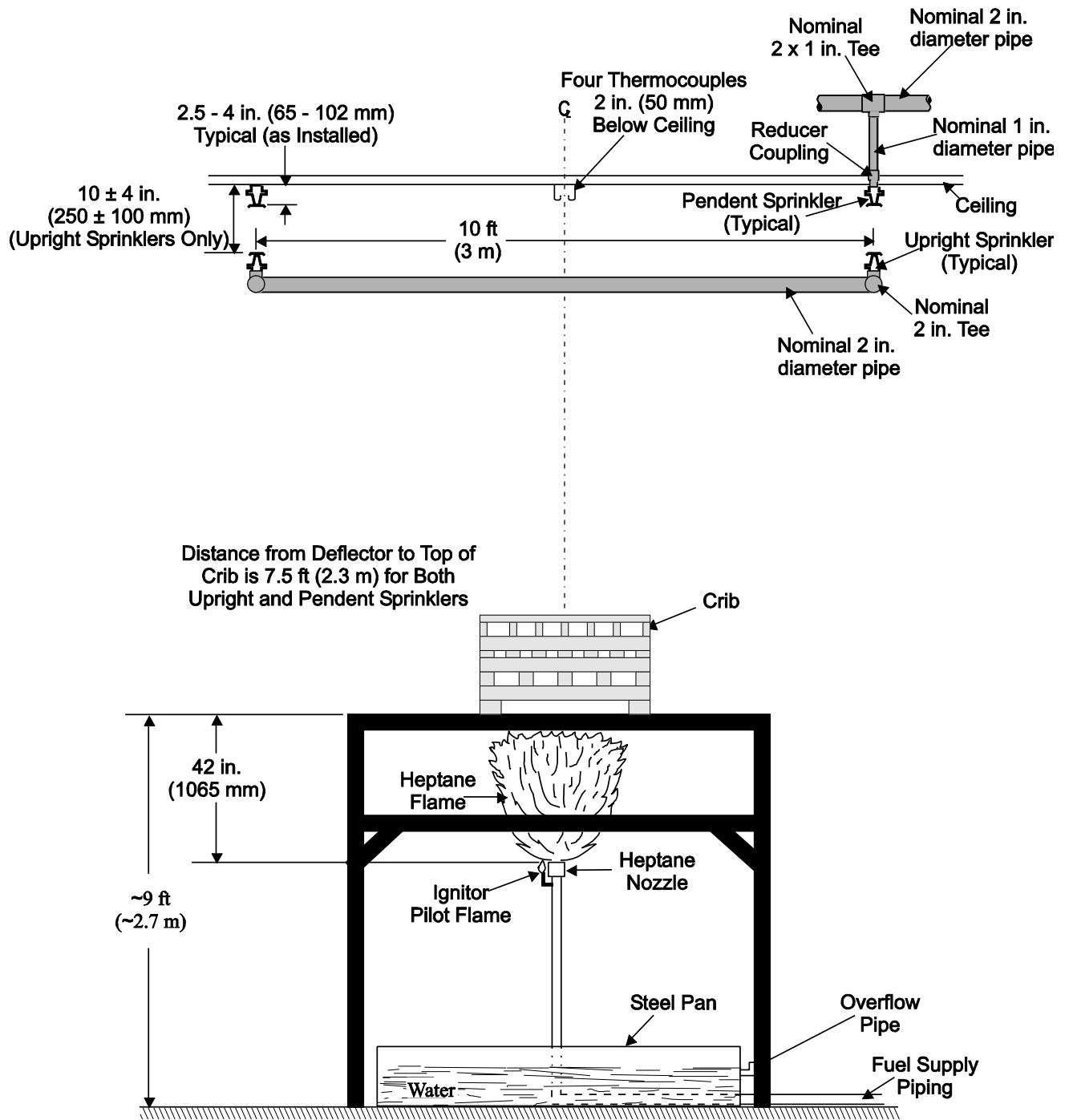
D-23: Crib Fire Test - Arrangement with Piping
