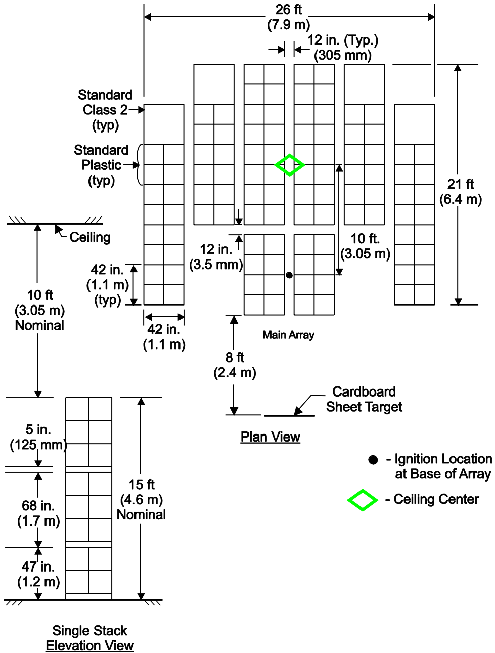
D-26: Full Scale Fire Test Array for K14.0 (K200) Upright and Pendent Storage Sprinklers, Test C
