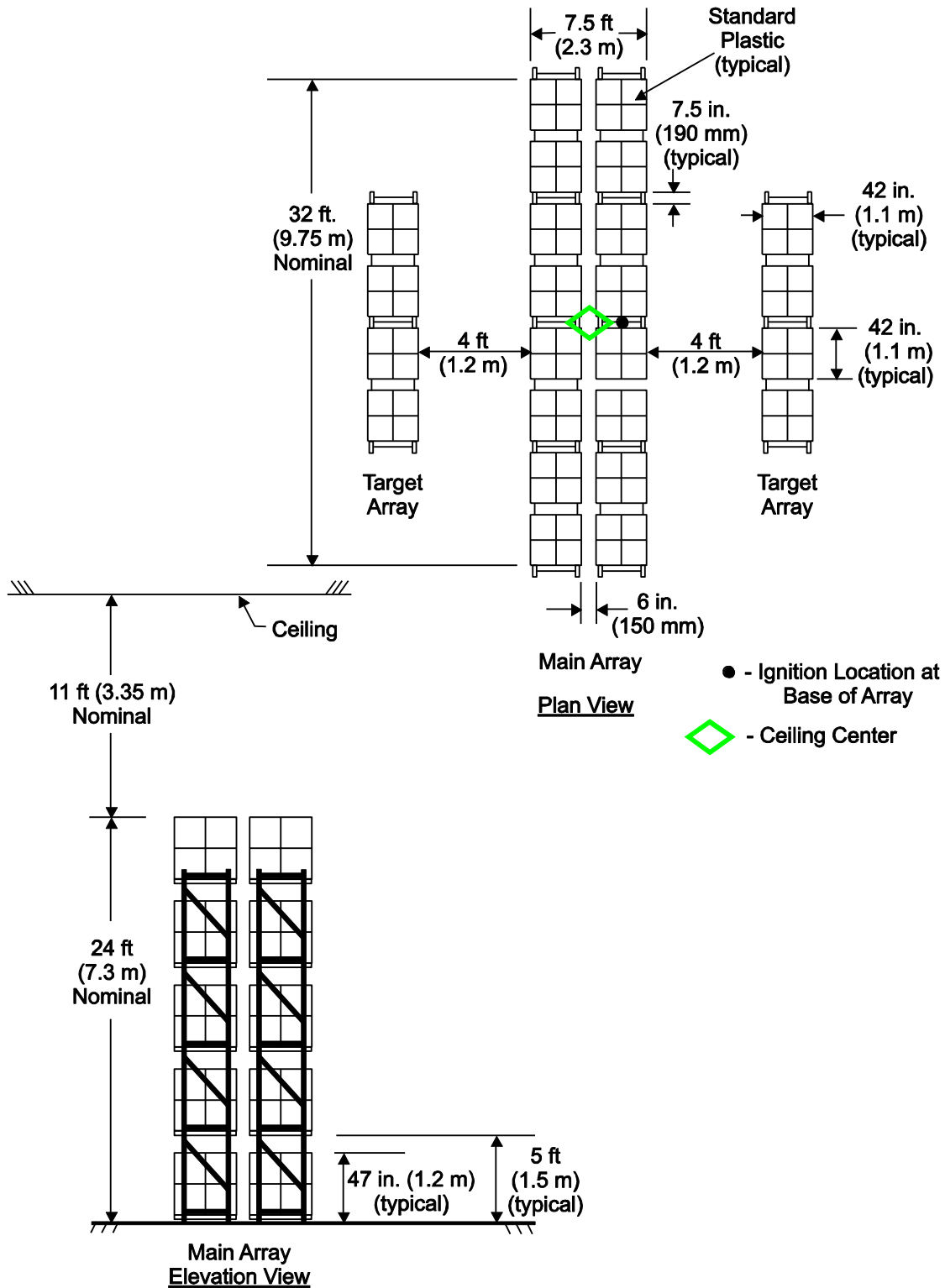
D-37: Full Scale Fire Test Array for K19.6 (K280) Pendent Sprinkler, Test D and E
