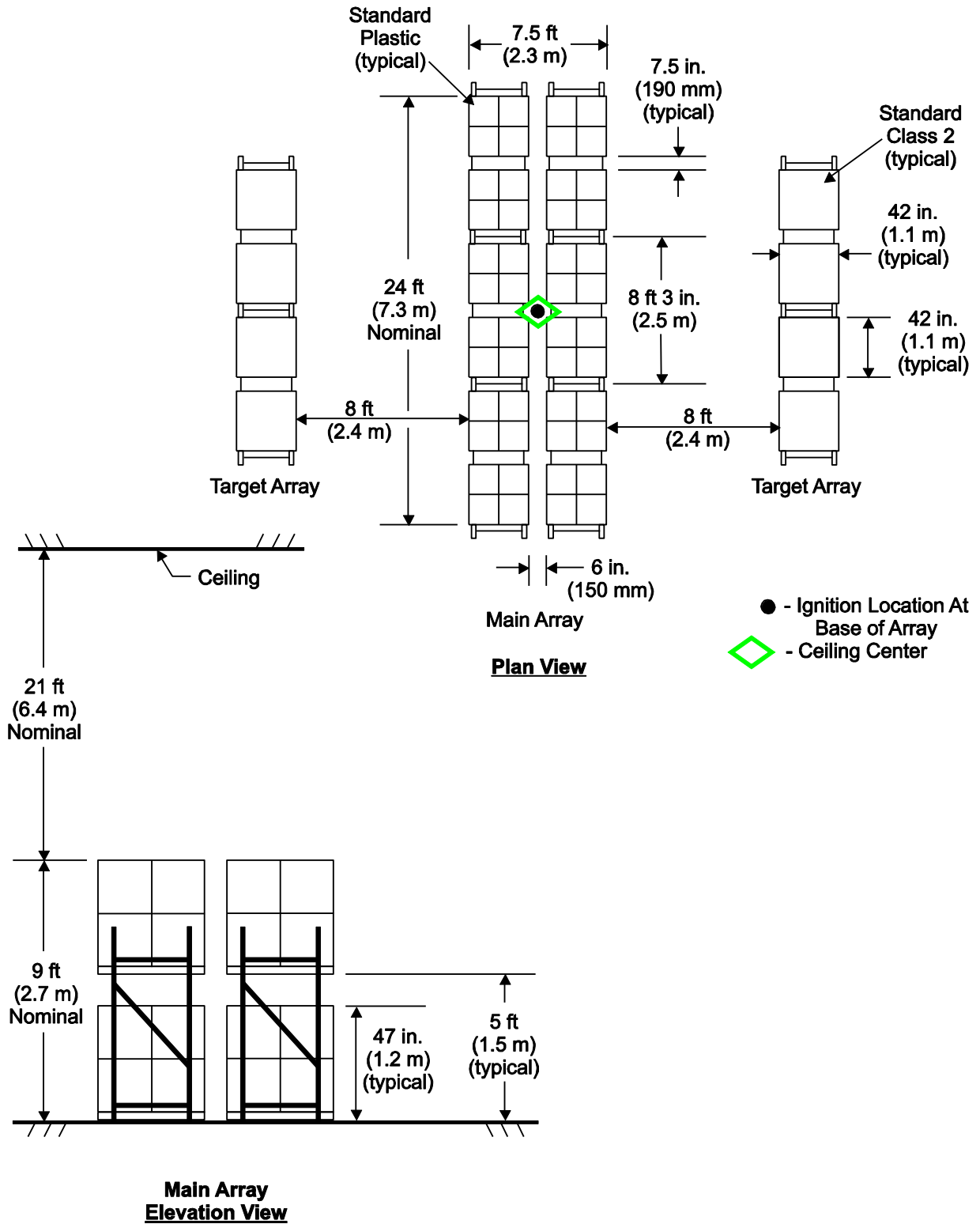
D-33: Full Scale Fire Test Array for K16.8 (K240) Upright Storage Sprinkler, Test A
