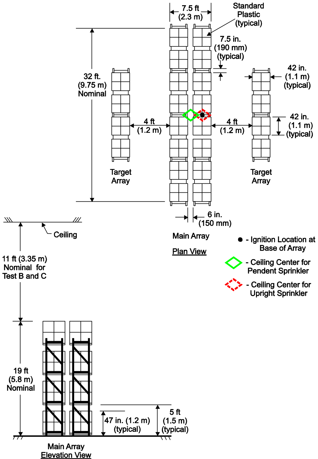
D-42: Full Scale Fire Test Array for K25.2 EC (K360EC) Upright and Pendent Sprinklers, Test B and C
