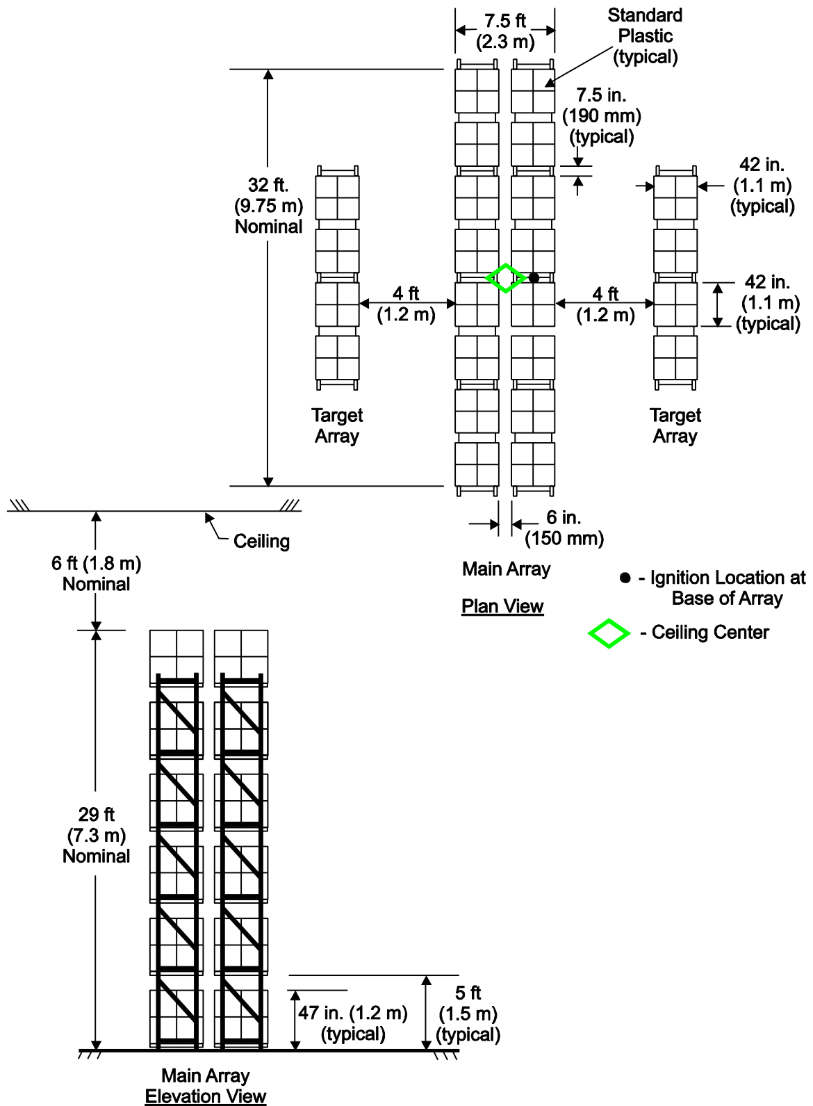
D-38: Full Scale Fire Test Array for K19.6 (K280) Pendent Sprinkler, Test F
