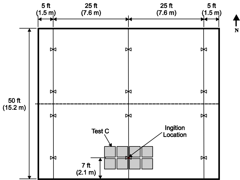
D-31: Array Positions for Screening Tests of K14.0 (K200) Non-Storage Extended Coverage Horizontal Sidewall Sprinkler
