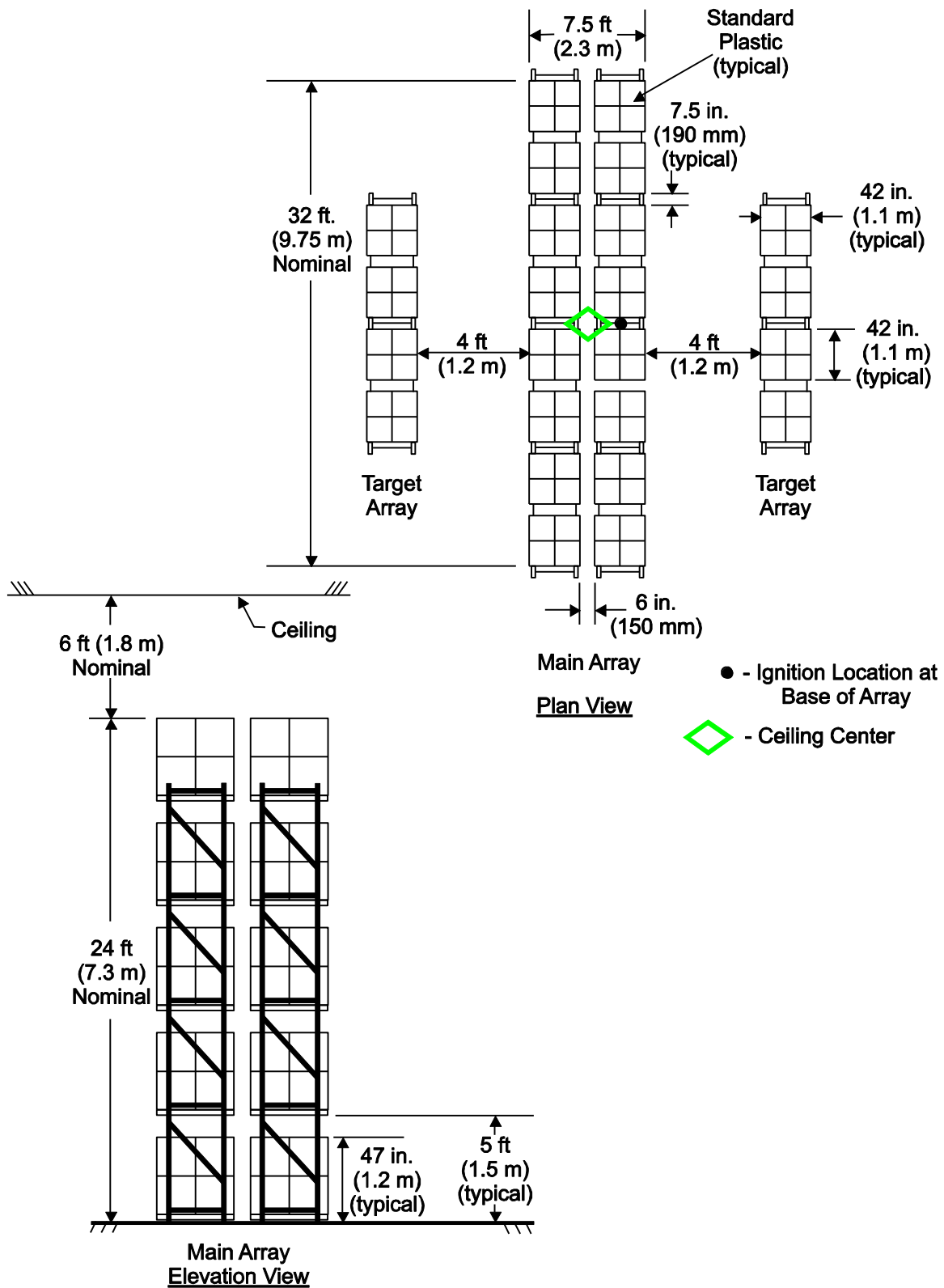
D-41: Full Scale Fire Test Array for K25.2 EC (K360EC) Upright and Pendent Sprinklers, Test A
