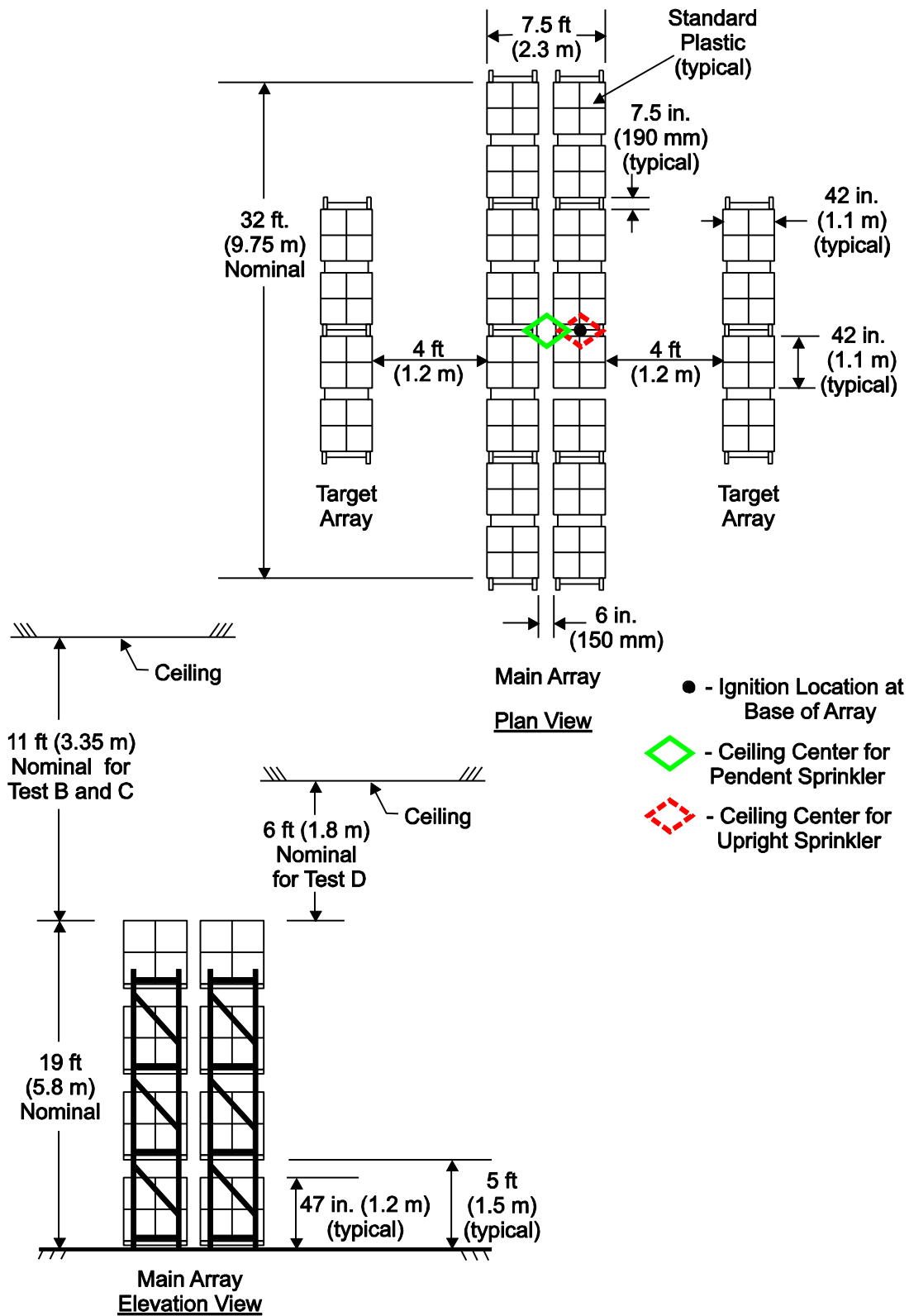
D-40: Full Scale Fire Test Array for K25.2 (K360) Upright and Pendent Sprinklers, Test B and C
