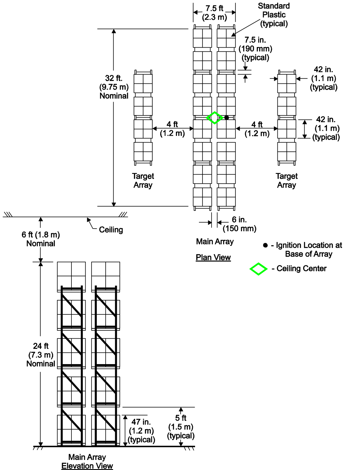
D-39: Full Scale Fire Test Array for K25.2 (K360) Upright and Pendent Sprinklers, Test A
