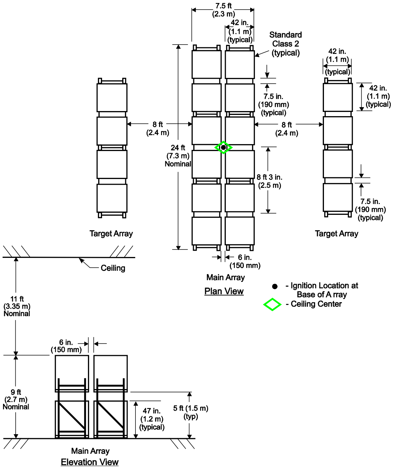
D-27: Full Scale Fire Test Array for K14.0 (K200) Extended Coverage Hazard Category 1-3 Sprinkler
