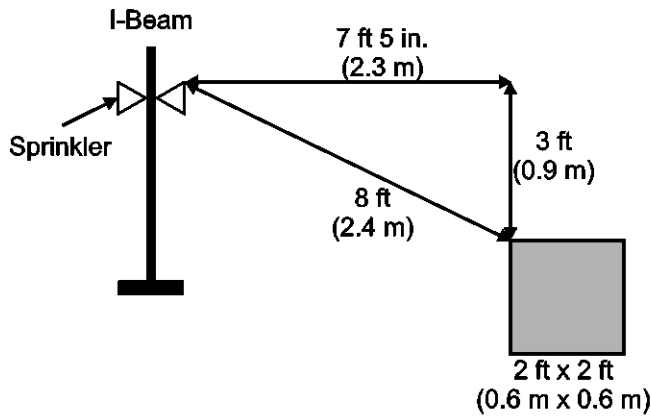
End Elevation View 2 ft (0.6 m) Wide Obstruction 8 ft (2.4 m) Separation
